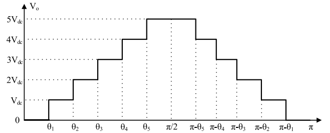
FIGURE 10. 11 level staircase output voltage waveform.
