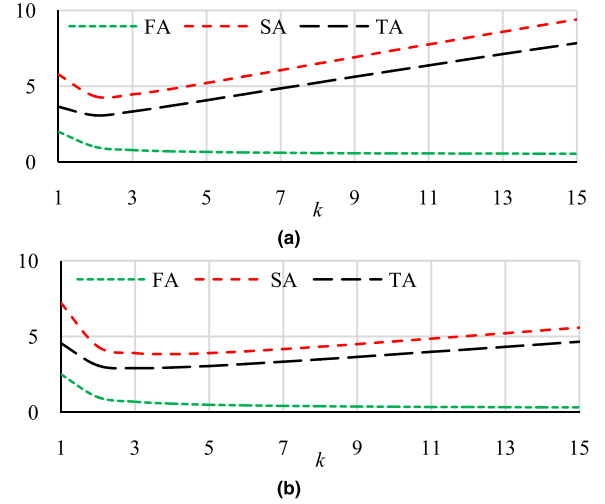
FIGURE 6. Curves related to optimization for (a) minimization of switches and (b) minimization of driver circuit with constant number of levels.
